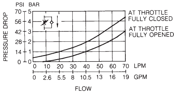
PRESSURE DROP FOR FREE FLOW
