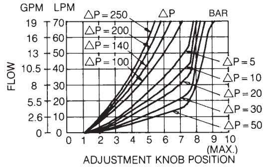
METERED FLOW VS. DIAL POSITION
