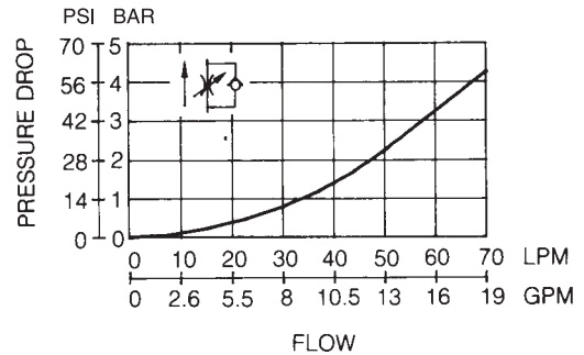
PRESSURE DROP AT THROTTLE FULLY OPENED
