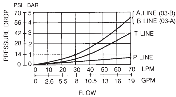
PRESSURE DROP
